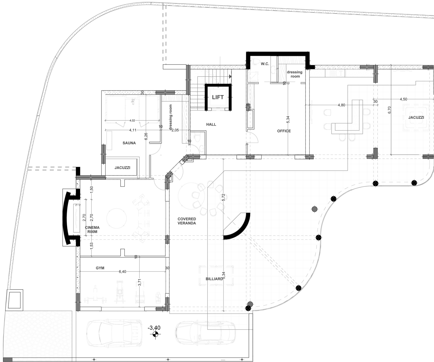
Eagle Residence - Basement Level 2
